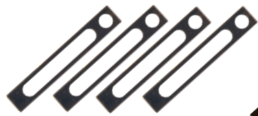
T50505 (x4) STRAIGHT EDGE STOP, 6.0" X 1.18" X 0.47"
